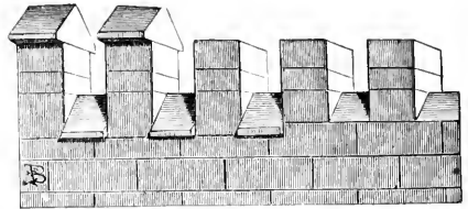
Fig. 77. Battlement.
